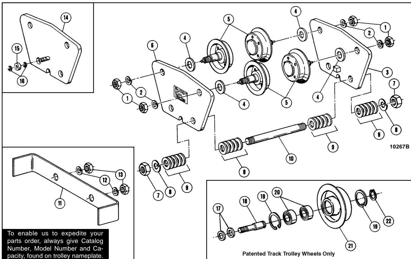
Figure 3. Push Type Rigid Mount Trolley Assembly - ( \frac{1}{2} , 1, 1\frac{1}{2} , 2 & 3 Ton Rated Loads)
